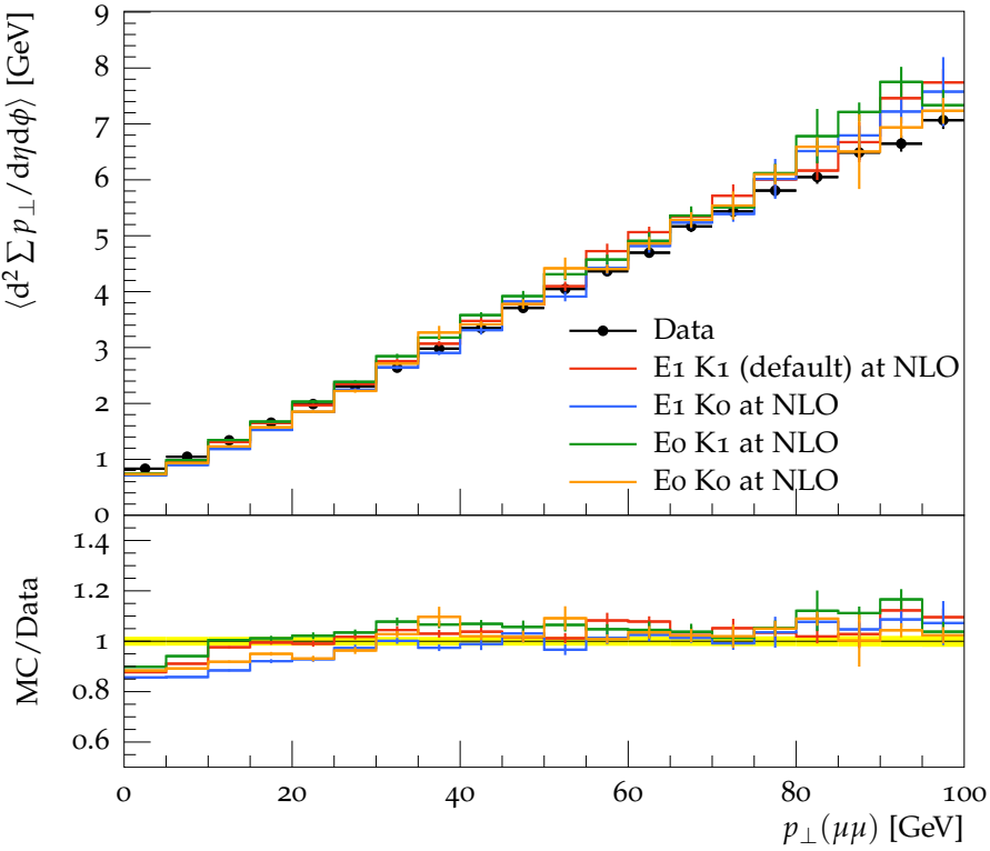
Away \Sigma p_{\perp} density vs p_{\perp}^{\mu\mu}
