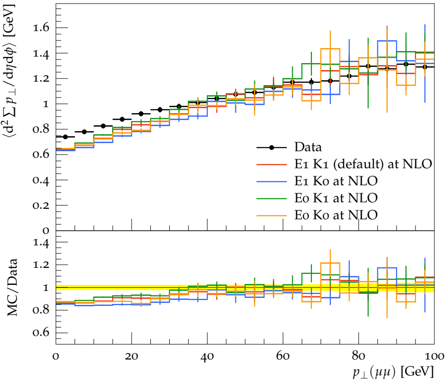
Toward \Sigma p_{\perp} density vs p_{\perp}^{\mu\mu}
