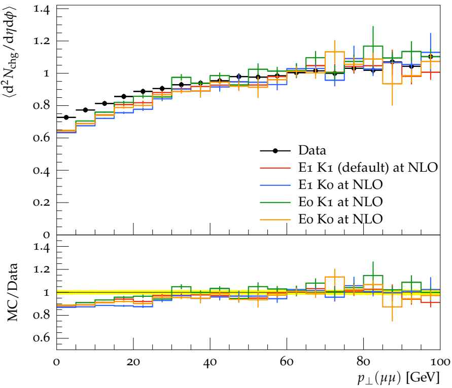
Transverse N_{\text{chg}} density vs p_{\perp}^{\mu\mu}
