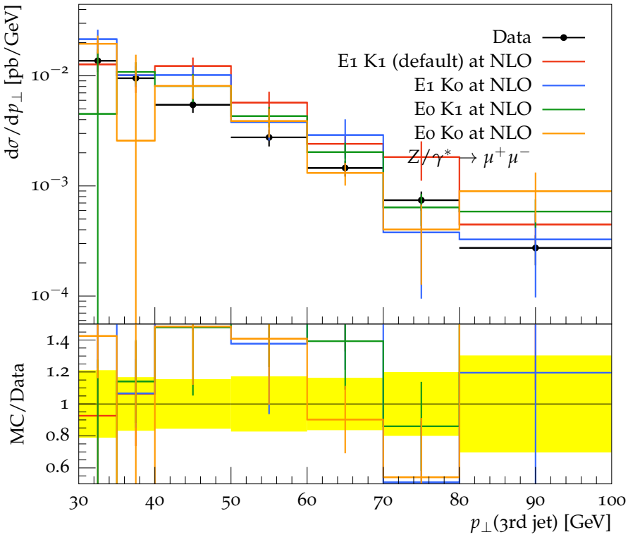
Transverse momentum of 3rd jet (VBF selection)
