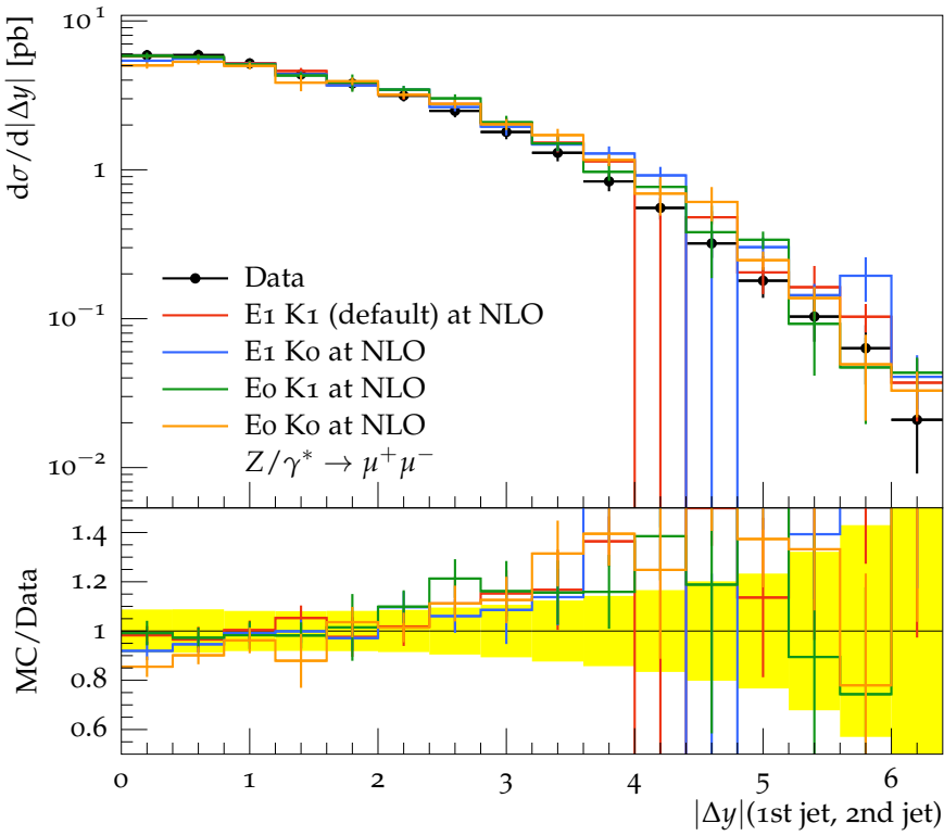
Rapidity distance of leading jets
