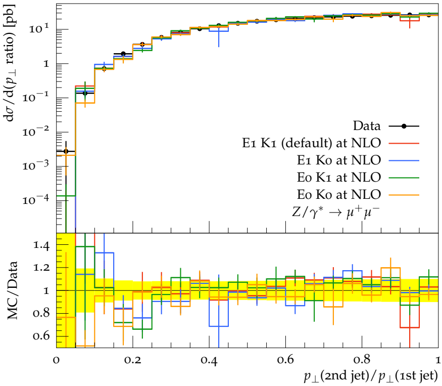
Ratio of jet transverse momenta
