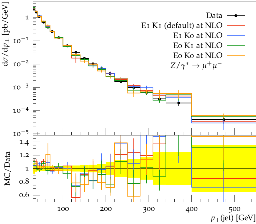
Transverse jet momentum in Z + 1\text{jet} events
