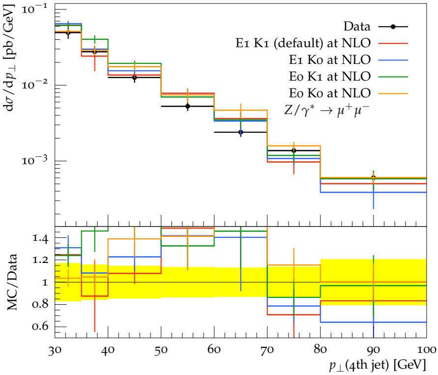
Transverse momentum of 4th jet
