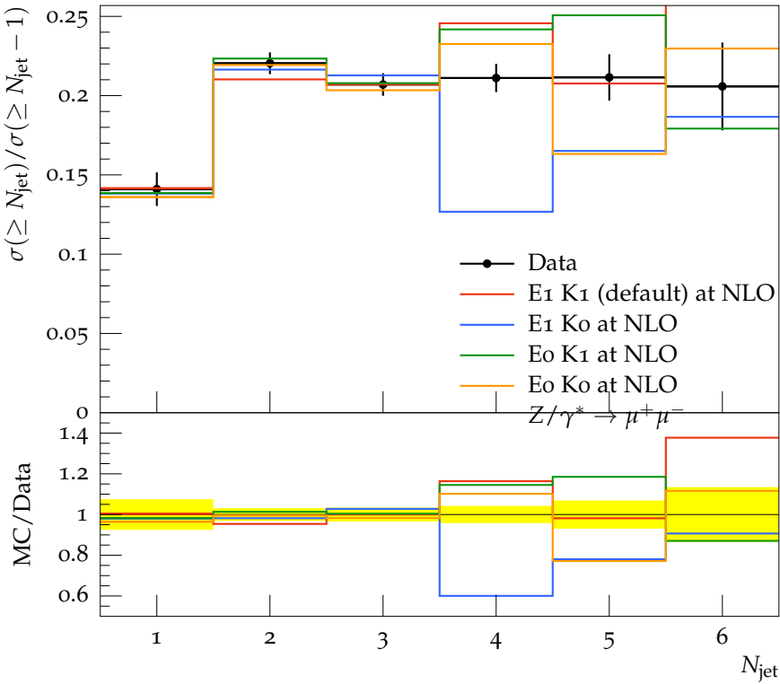
Inclusive jet multiplicity ratio
