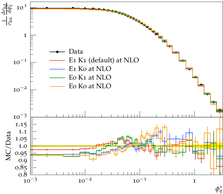
\phi_\eta^* spectrum, Z \rightarrow \mu\mu (dressed)
