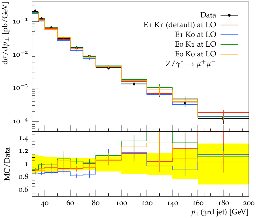
Transverse momentum of 3rd jet
