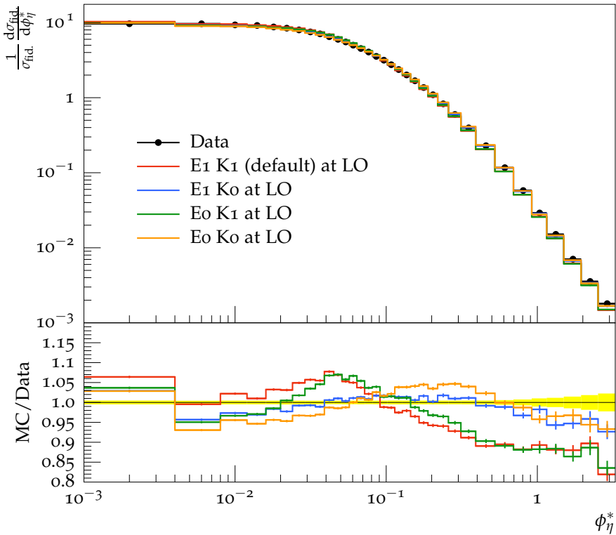
\phi_\eta^* spectrum, Z \rightarrow \mu\mu (dressed)
