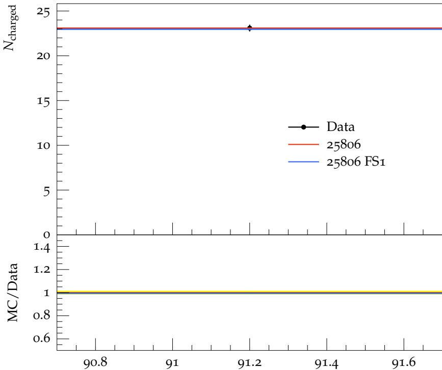
Charged particle multiplicity, b events
