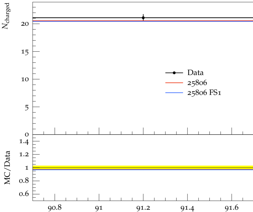
Charged particle multiplicity, c events
