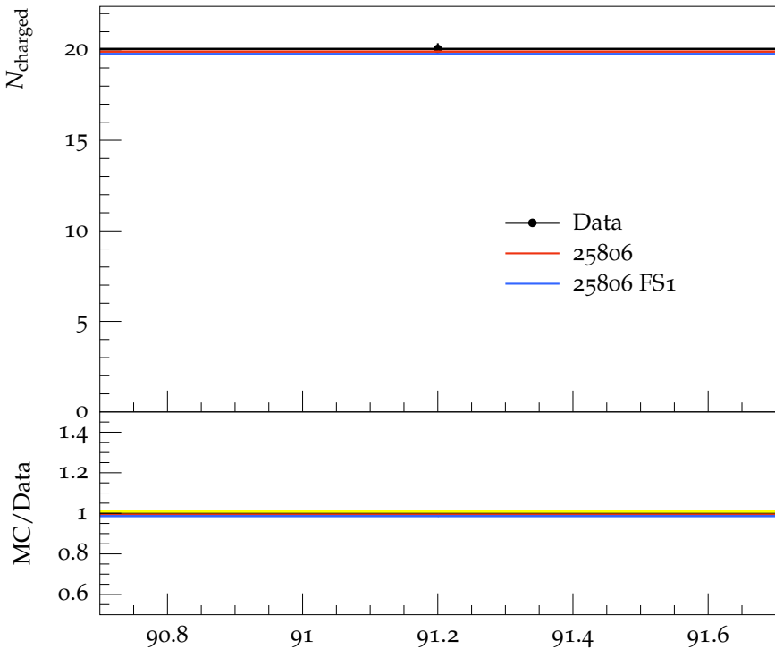
Charged particle multiplicity, ( uds ) events
