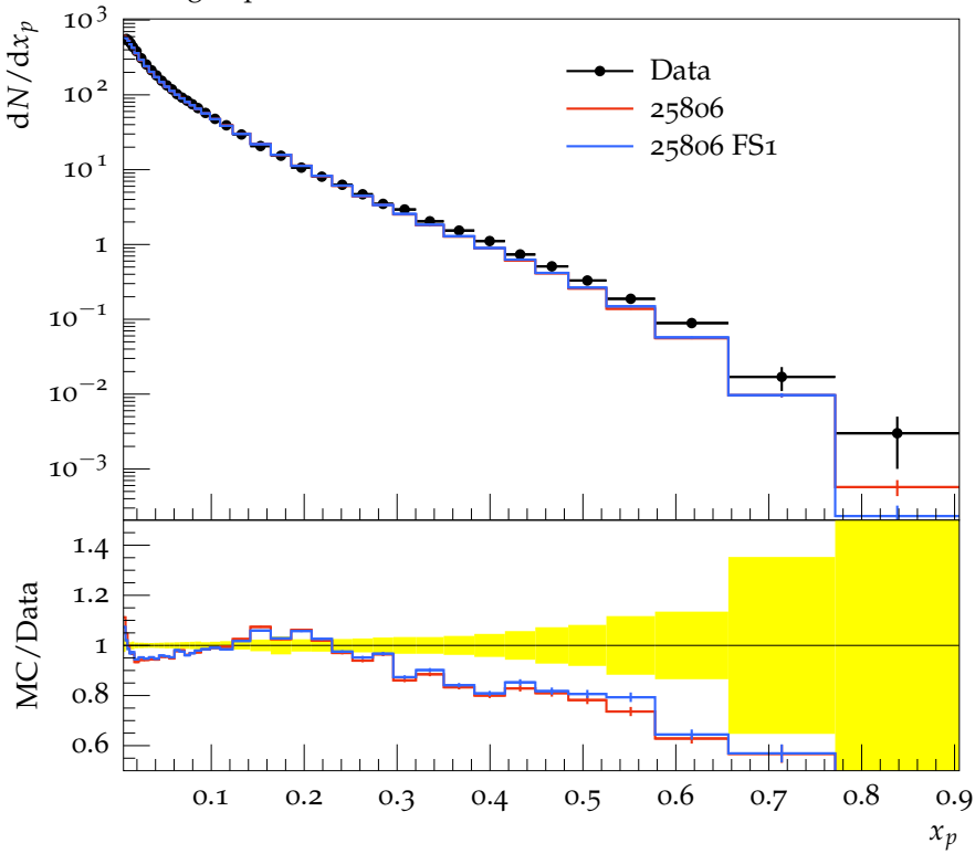
Charged particle scaled Momentum, b events
