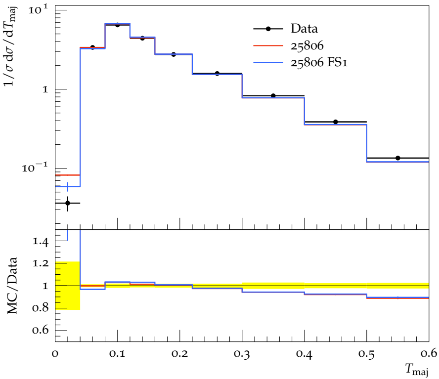
Thrust major, T_{maj} , at 91 GeV
