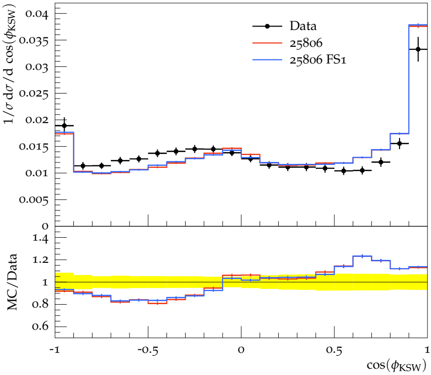
Körner-Schierholz-Willrodt \cos(\phi_{\text{KSW}}) , Jade y_{\text{cut}} = 0.015
