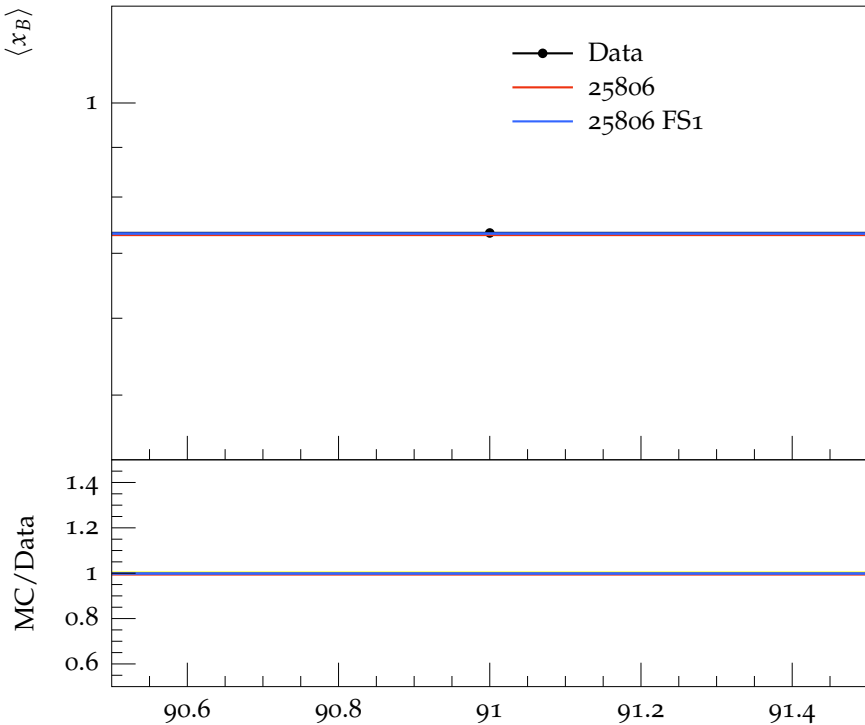
Mean of b quark fragmentation function f(x_B^{\text{prim}})
