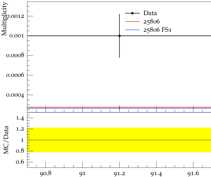
Mean \Omega^\mp multiplicity
