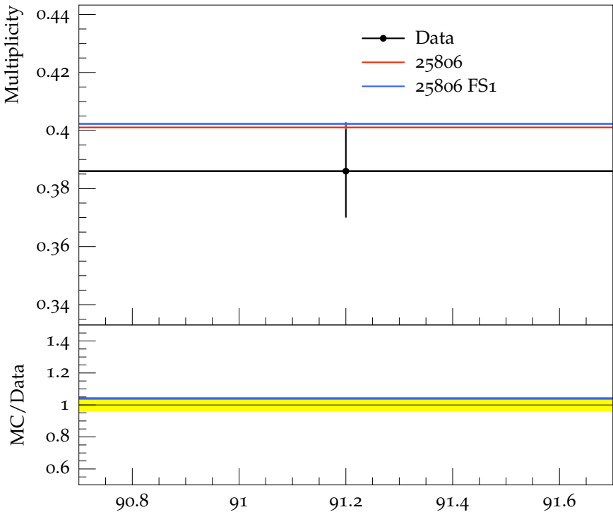
Mean \Lambda multiplicity
