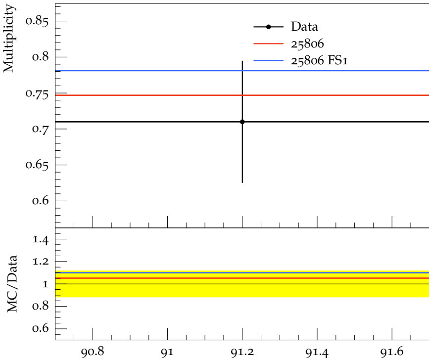
Mean K^{*\pm} multiplicity
