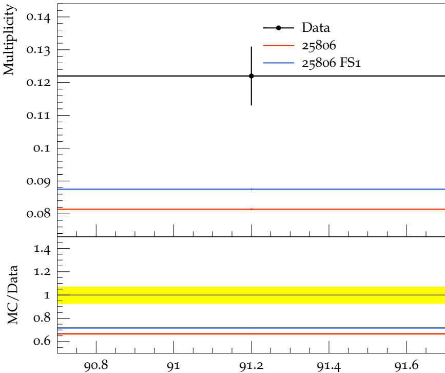
Mean \phi multiplicity
