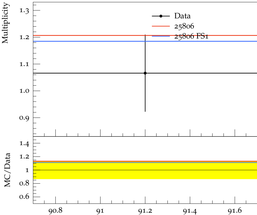
Mean \omega(782) multiplicity
