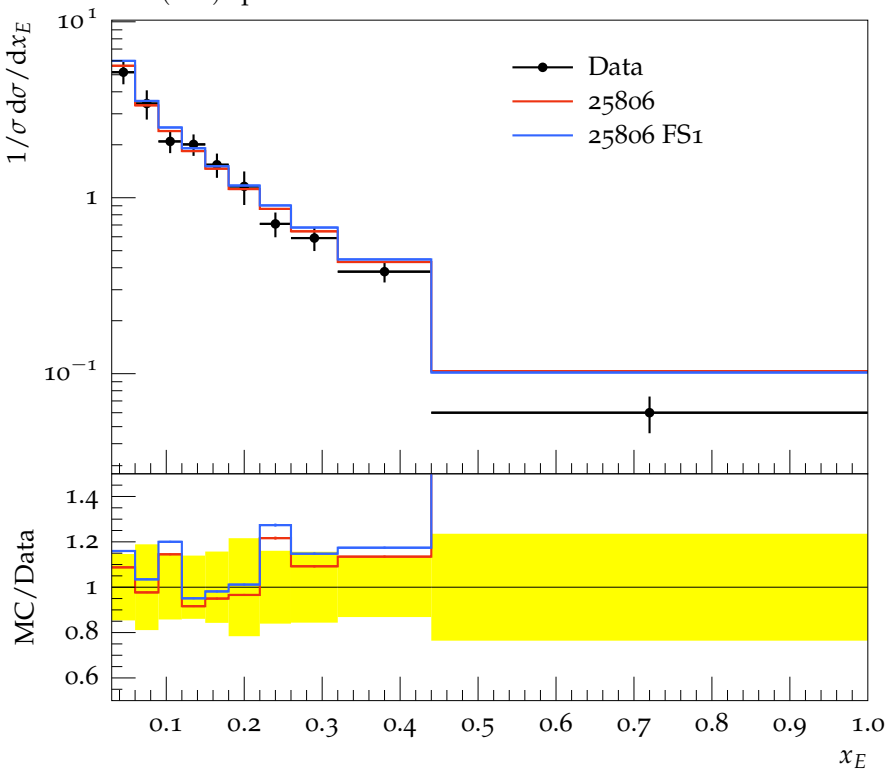
K^{*\pm}(892) spectrum
