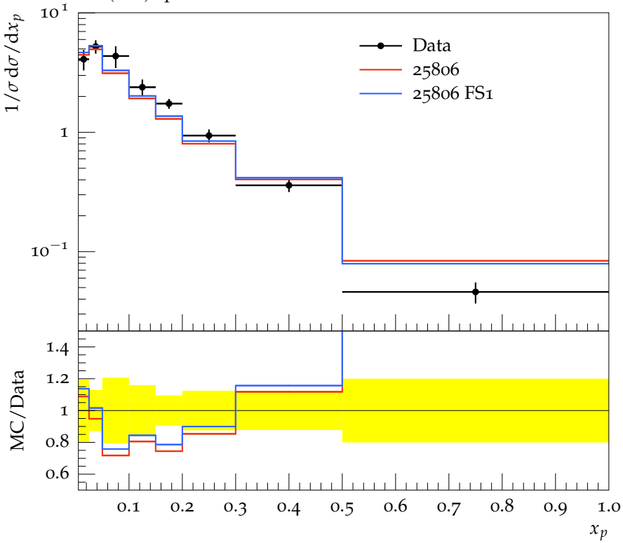
K^{*0}(892) spectrum
