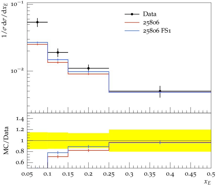
\Xi^0(1530) spectrum
