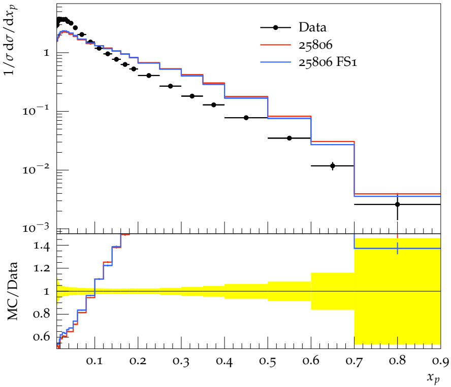
\Lambda^0 spectrum
