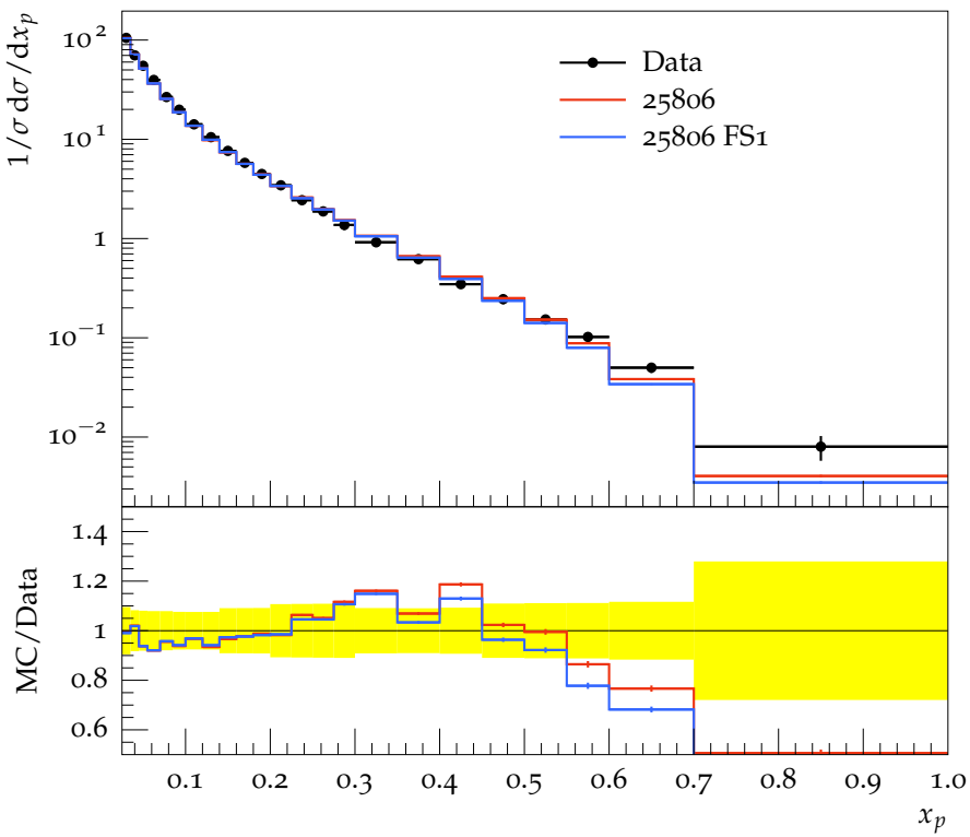
\pi^0 spectrum
