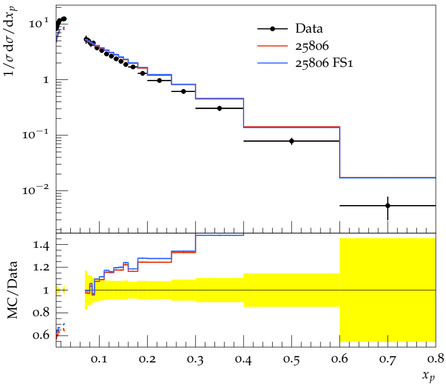
p spectrum
