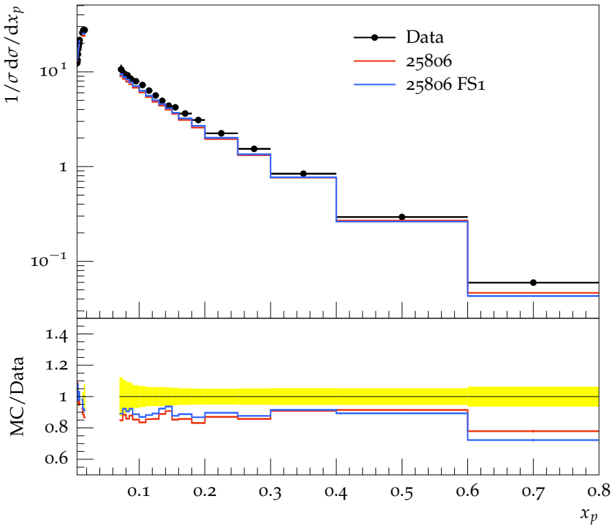
K^\pm spectrum
