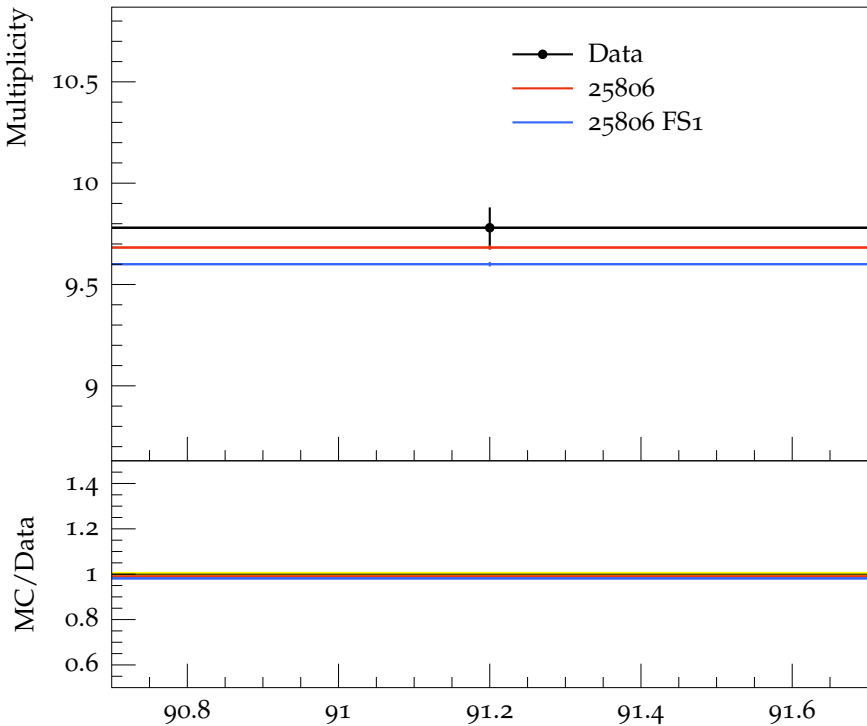
Mean charged multiplicity for rapidity |Y| < 1.5
