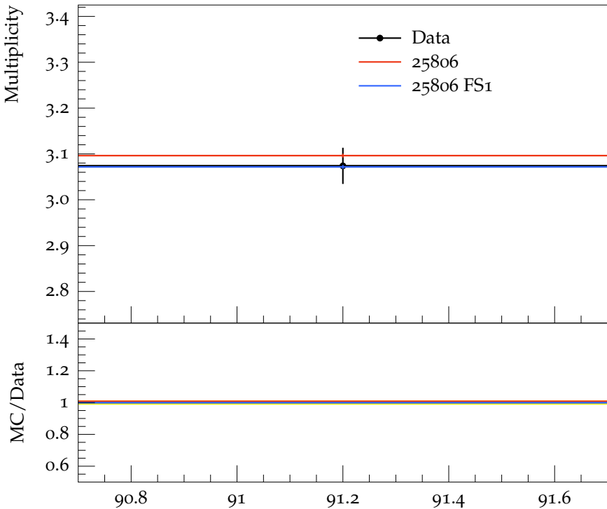
Mean charged multiplicity for rapidity |Y| < 0.5
