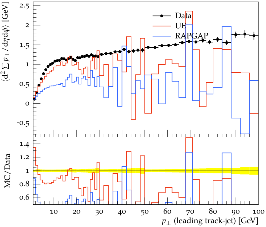
Transverse \Sigma p_{\perp} density vs. p_{\perp}^{\text{jet } 1} , \sqrt{s} = 7000 GeV
