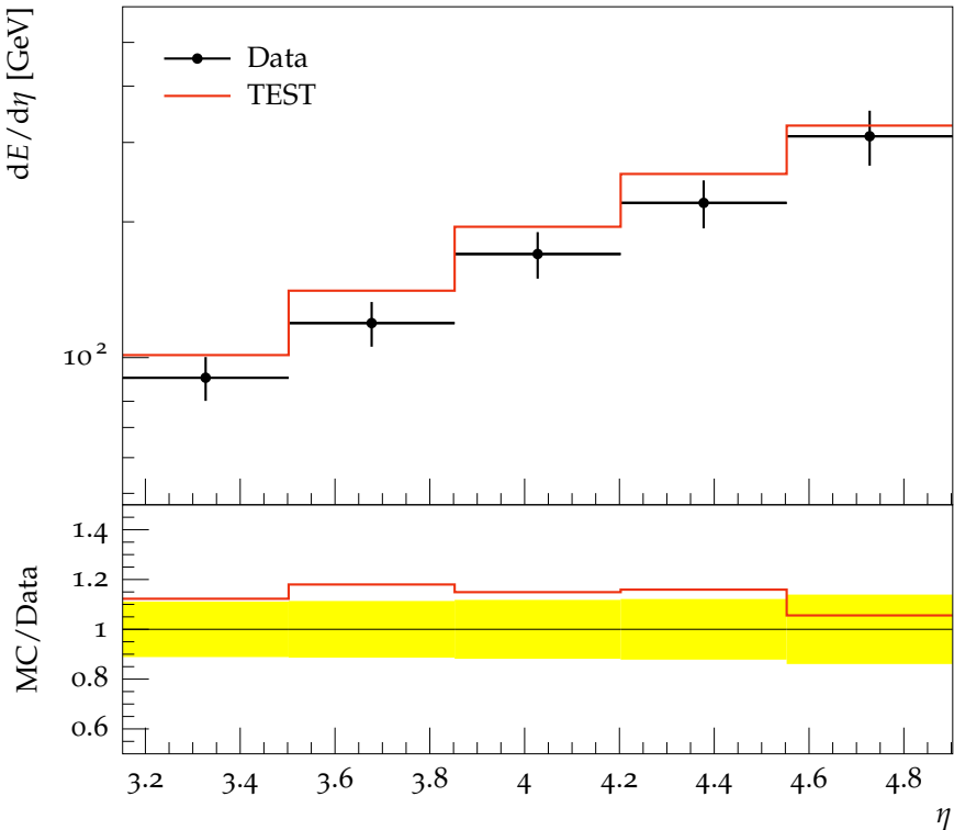
Energy flow in MB events, \sqrt{s} = 7 TeV
