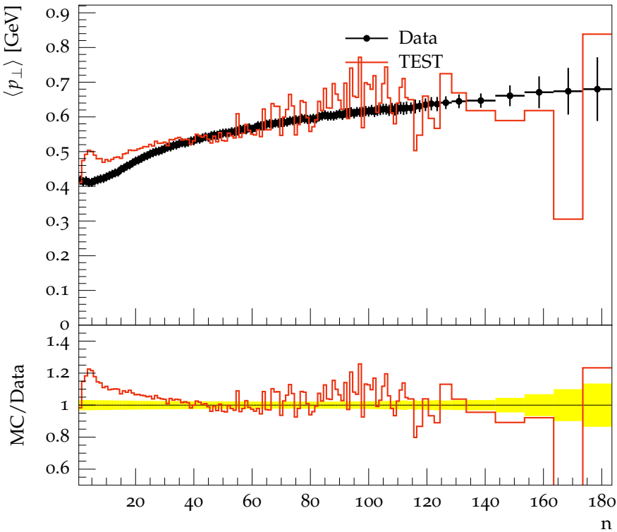
Mean p_{\perp} vs charged hadron multiplicity, |\eta| < 2.4 , \sqrt{s} = 7 TeV
