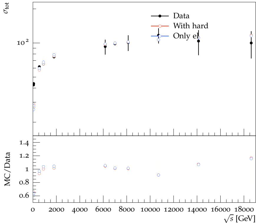
Total cross section vs \sqrt{s}
