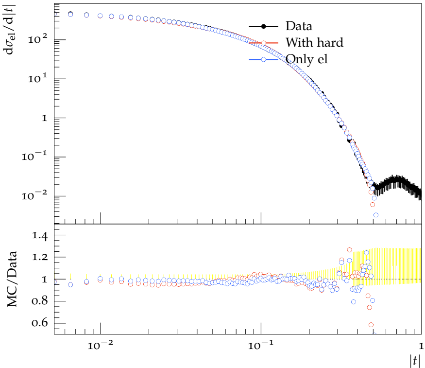
Elastic cross section vs |t| at \sqrt{s} = 7000 GeV
