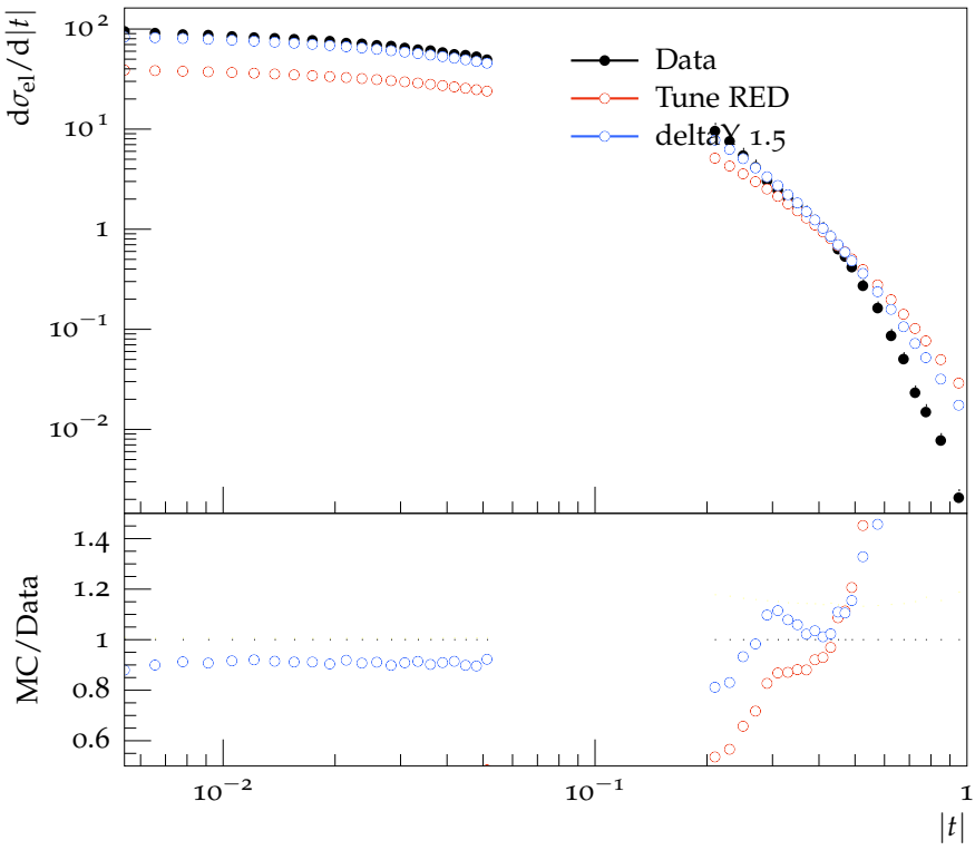
Elastic cross section vs |t| at \sqrt{s} = 62.5 GeV
