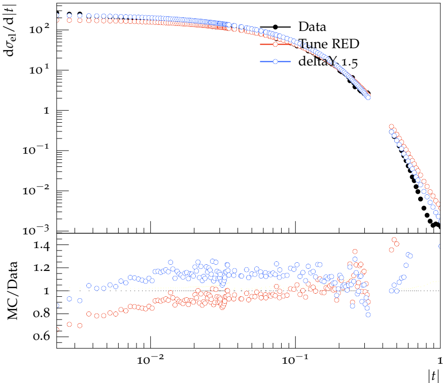
Elastic cross section vs |t| at \sqrt{s} = 546 GeV
