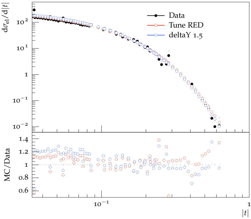
Elastic cross section vs |t| at \sqrt{s} = 1800 GeV
