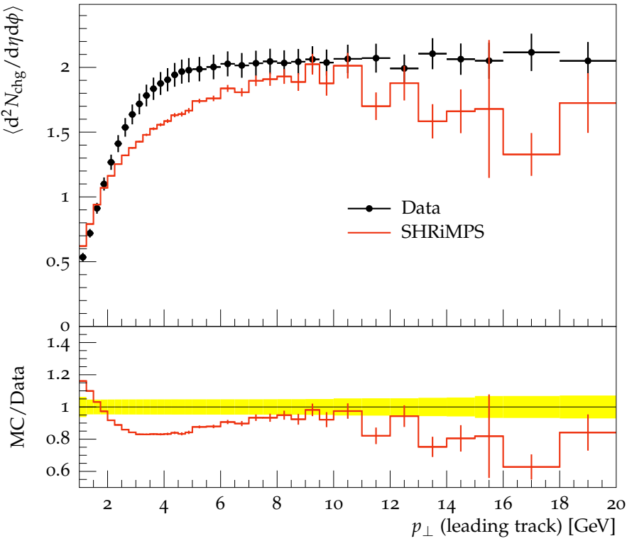
Transverse N_{\text{chg}} density vs. p_{\perp}^{\text{trk1}} , \sqrt{s} = 7 TeV, p_{\perp} > 100 MeV
