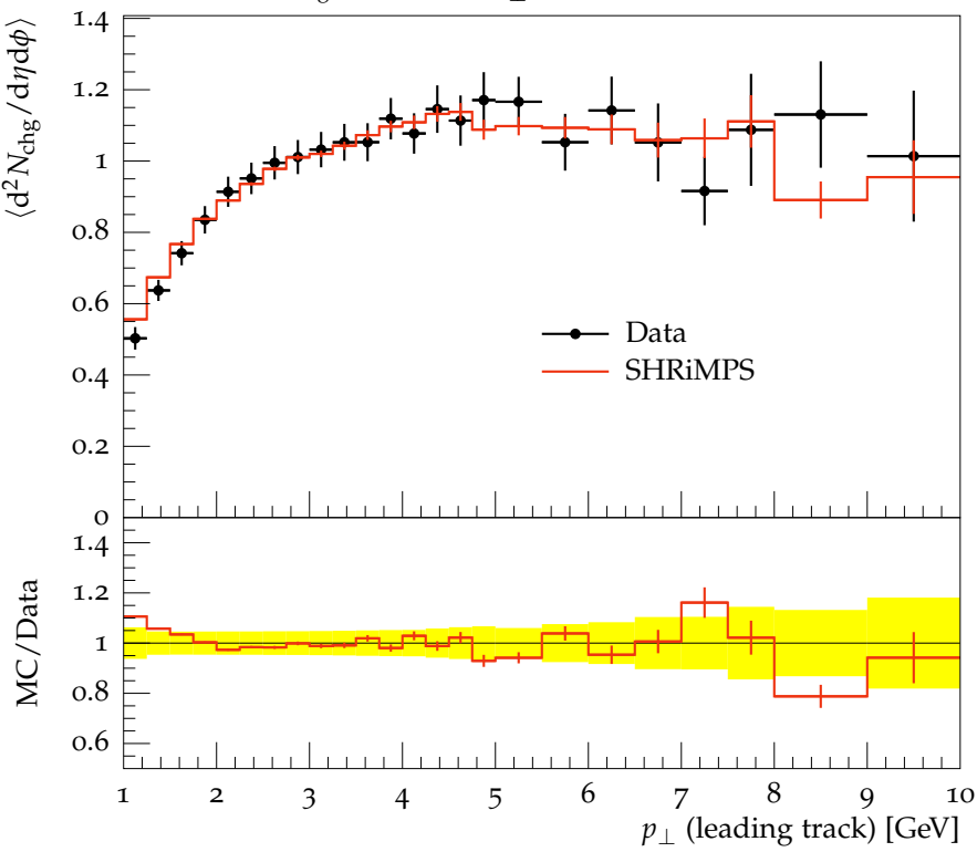
Transverse N_{\text{chg}} density vs. p_{\perp}^{\text{trk1}} , \sqrt{s} = 900 GeV, p_{\perp} > 100 MeV
