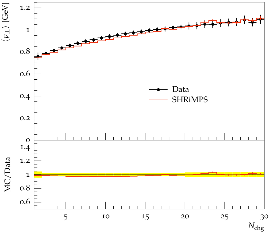
Transverse \langle p_{\perp} \rangle vs. N_{\text{chg}} , \sqrt{s} = 7 TeV
