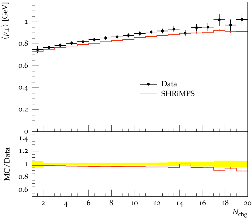
Transverse \langle p_{\perp} \rangle vs. N_{\text{chg}} , \sqrt{s} = 900 GeV
