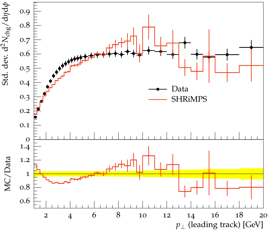
Std. dev. Transverse N_{\text{chg}} density vs. p_{\perp}^{\text{trk1}} , \sqrt{s} = 7 TeV
