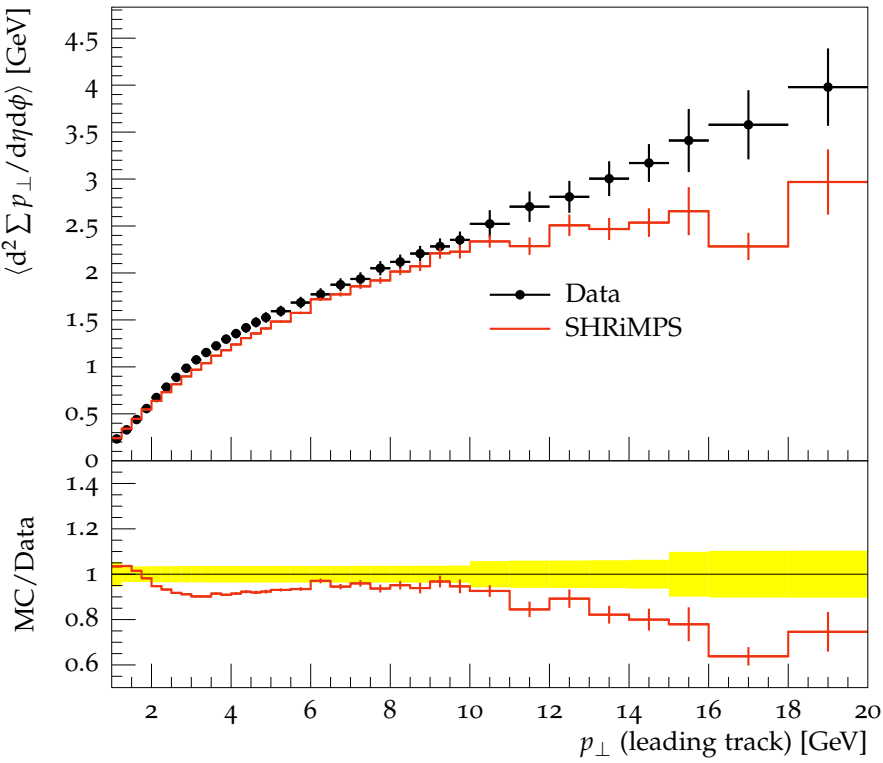
Toward \Sigma p_{\perp} density vs. p_{\perp}^{\text{trk1}} , \sqrt{s} = 7 TeV
