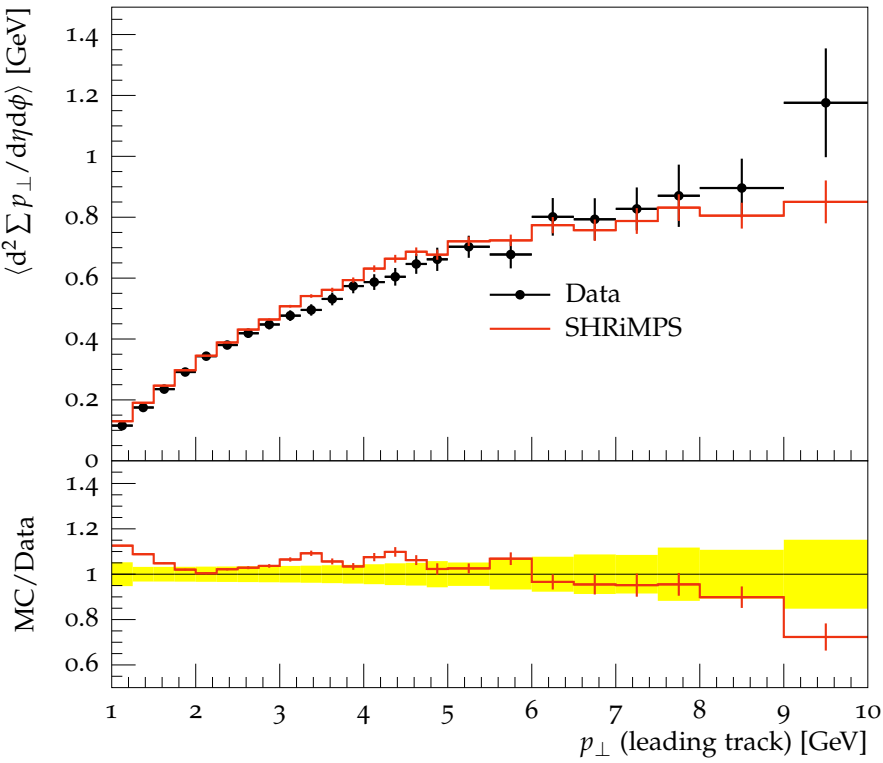
Away \Sigma p_{\perp} density vs. p_{\perp}^{\text{trk1}} , \sqrt{s} = 900 GeV
