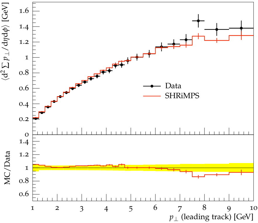
Toward \Sigma p_{\perp} density vs. p_{\perp}^{\text{trk1}} , \sqrt{s} = 900 GeV
