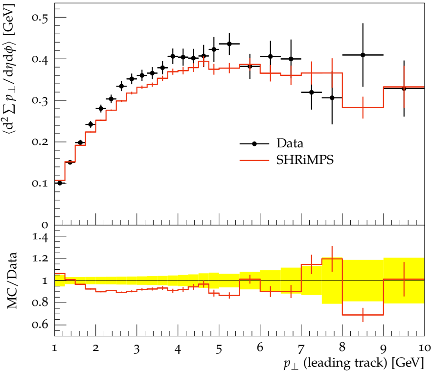
Transverse \Sigma p_{\perp} density vs. p_{\perp}^{\text{trk1}} , \sqrt{s} = 900 GeV
